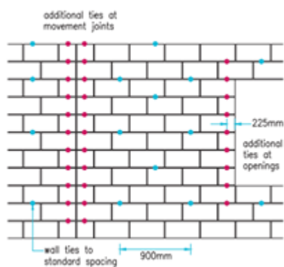
Figure 38: Wall tie locations
